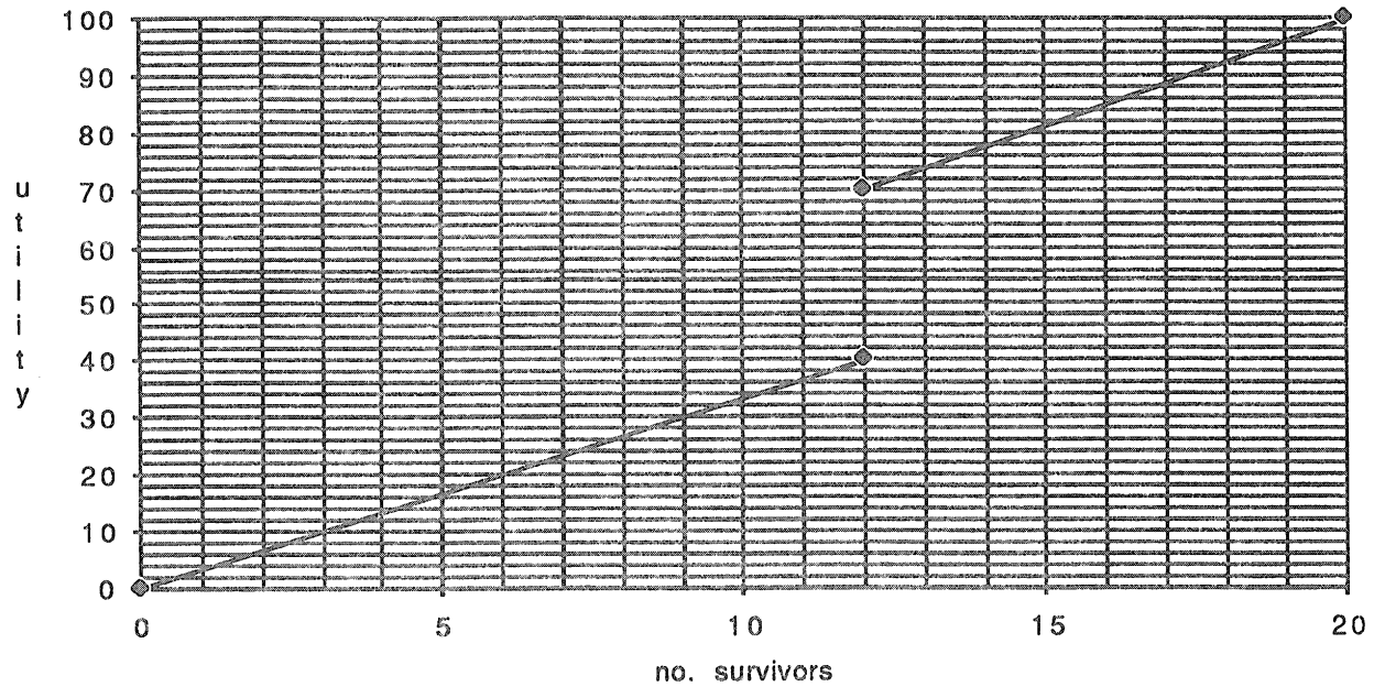
Utility Function
